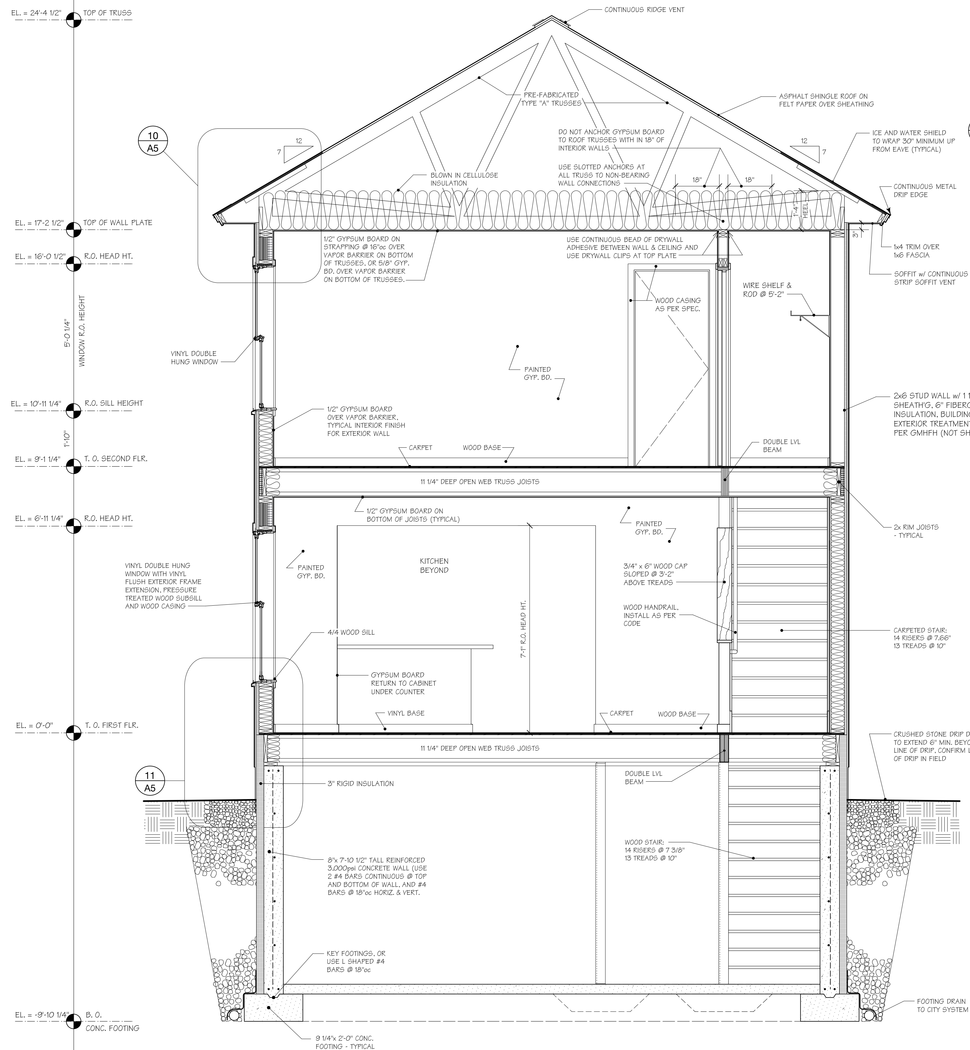
BUILDING SECTION - A 1/2" = 1' - 0"
