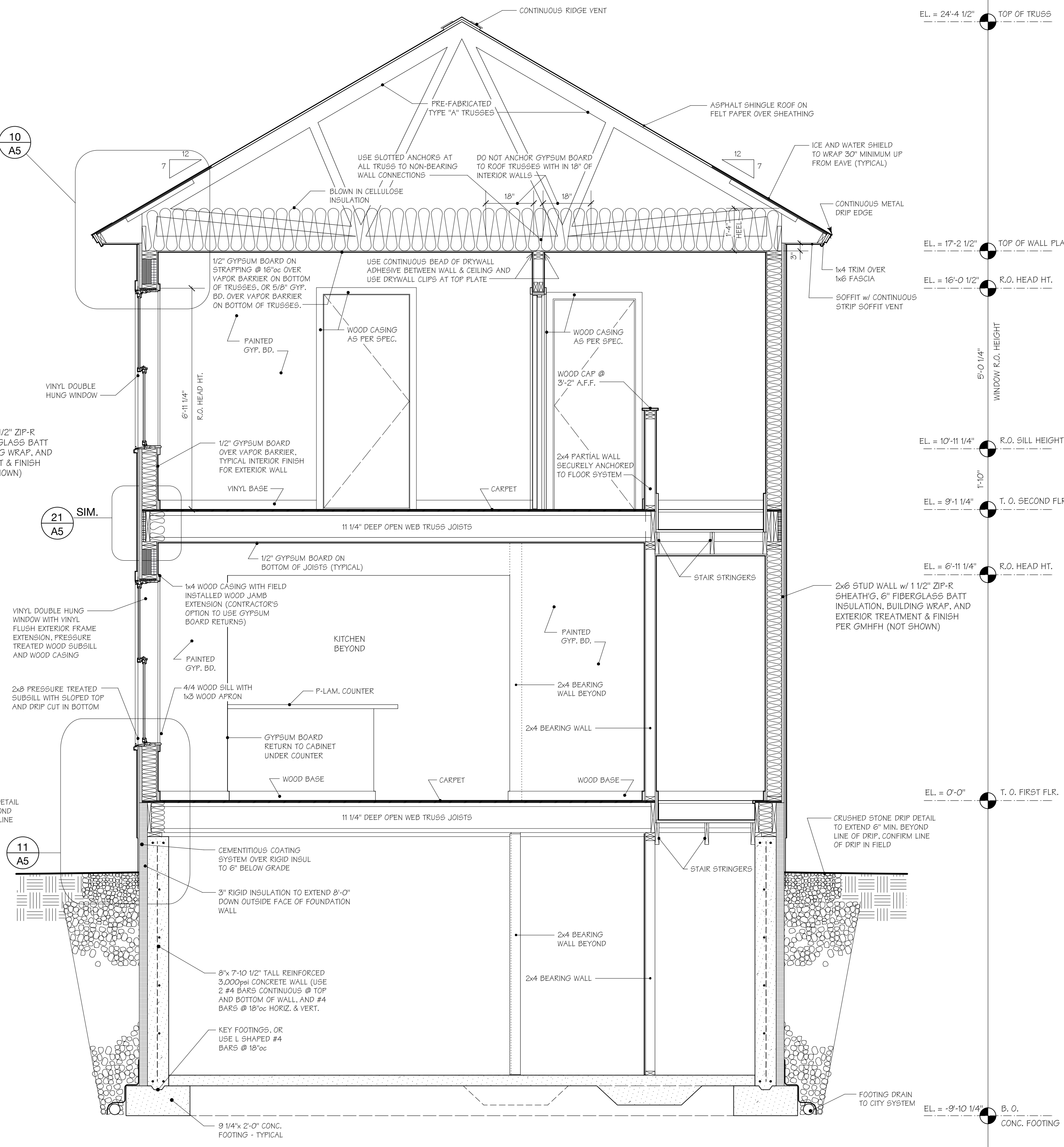
BUILDING SECTION - B 1/2" = 1' - 0"
