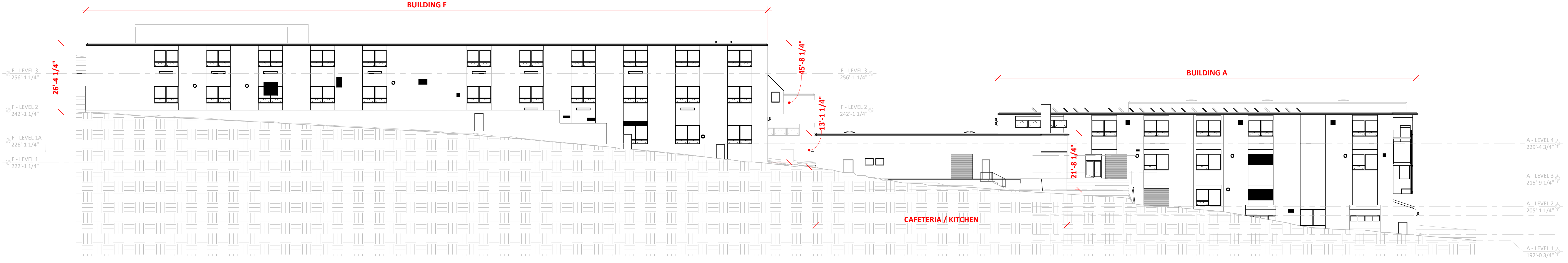
3 WEST - EXISTING OVERALL ELEVATION SCALE: 1/16" = 1'-0"
