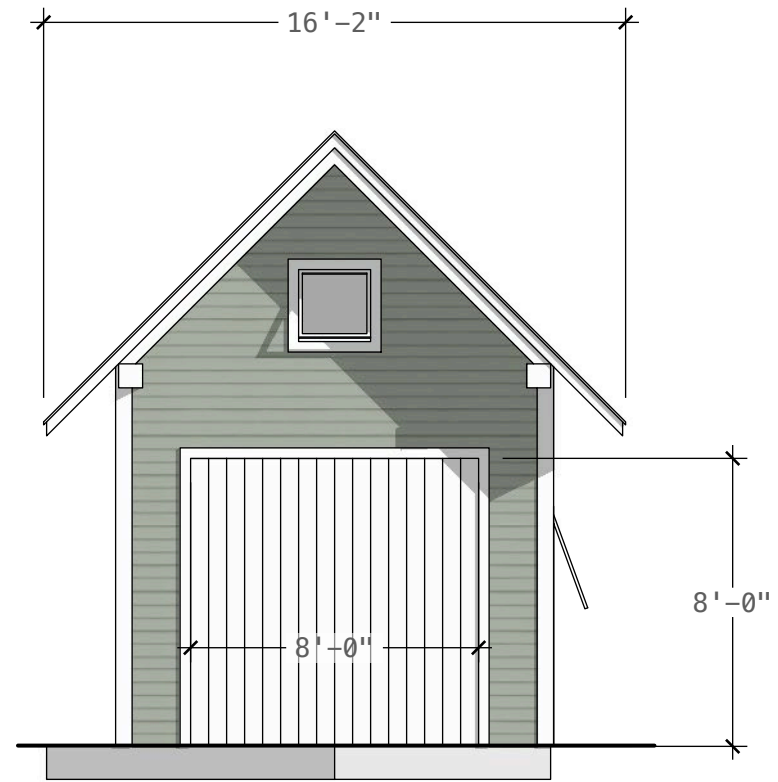
west elevation
