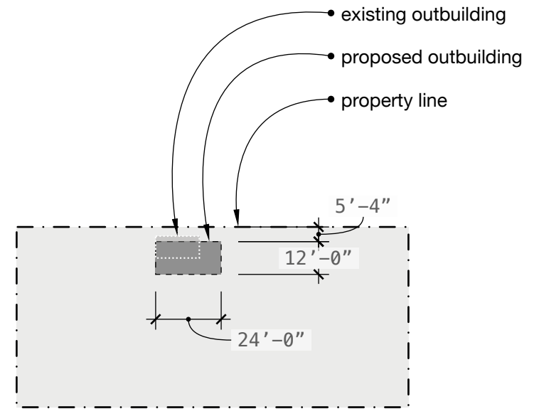
dimensioned site plan
