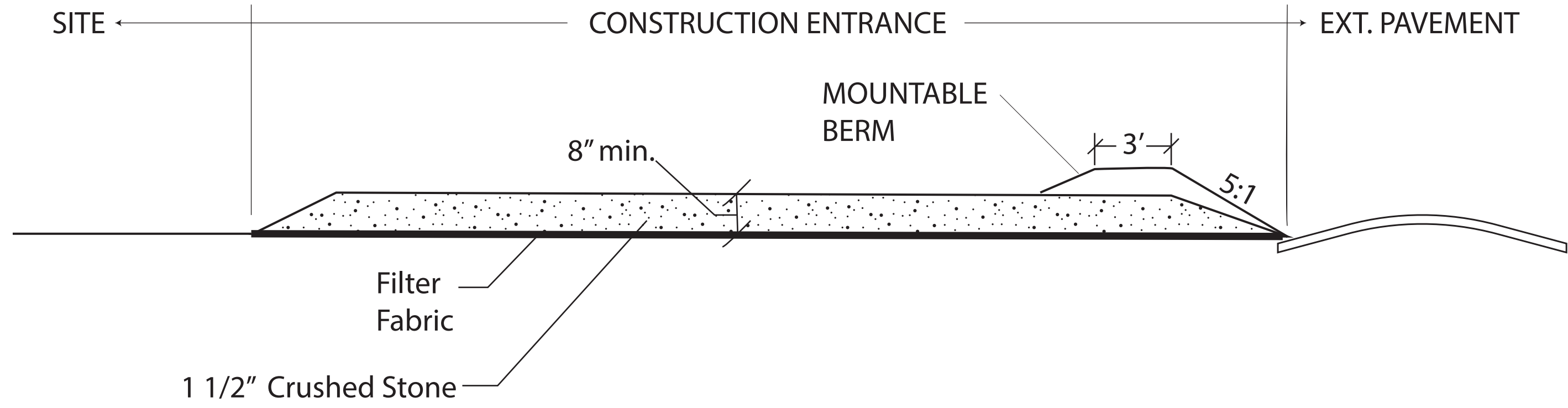
1 Stabilized Construction Entrance Section(N.T.S.)
