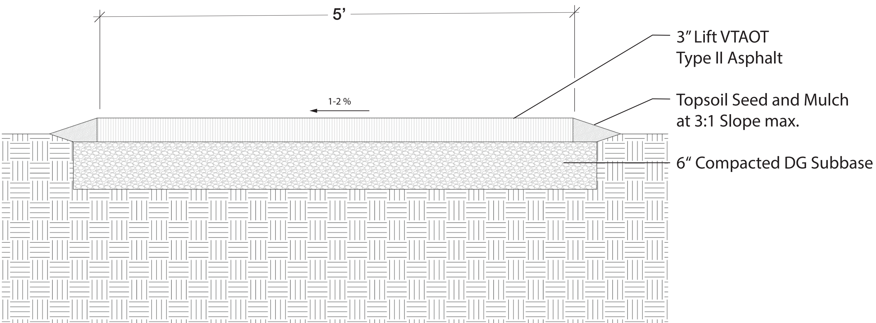
Asphalt Path Detail -Type II
