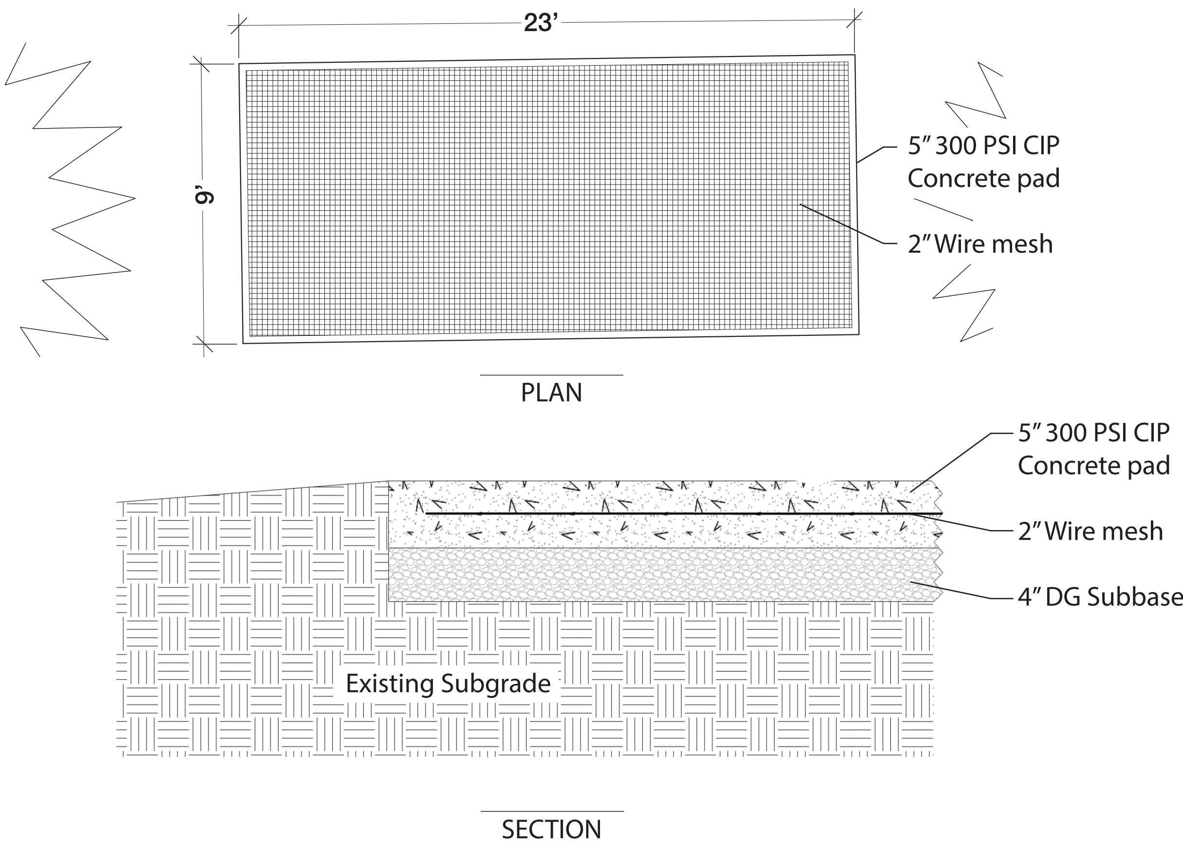
Concrete Bleacher Pad Detail
