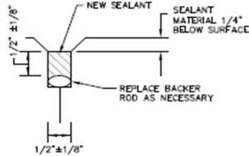
CONSTRUCTION/CONTRACTION JOINT NOT TO SCALE
