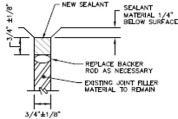
EXPANSION JOINT NOT TO SCALE
